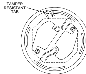
Figure 2. Detector mounting bracket:
