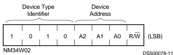
Slave Addresses (Figure 4).
