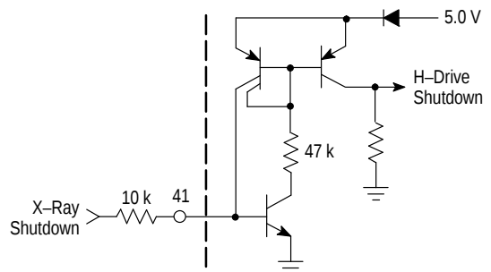
Figure 11. X-Ray Shutdown Circuit
