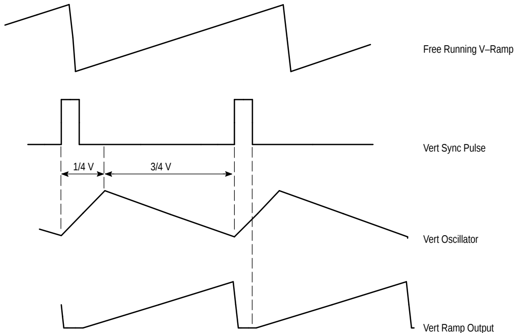
Figure 10. Vertical Section
