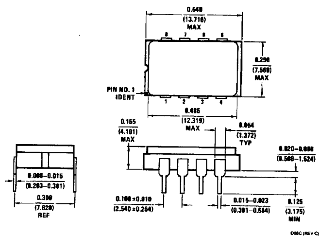
8-Pin Ceramic Sidebraced Dual-In-Line Package Order Number LM6142AMJ/883 NS Package Number D08C
