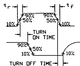
WAVEFORMS, CHANNEL BEING TURNED ON.
