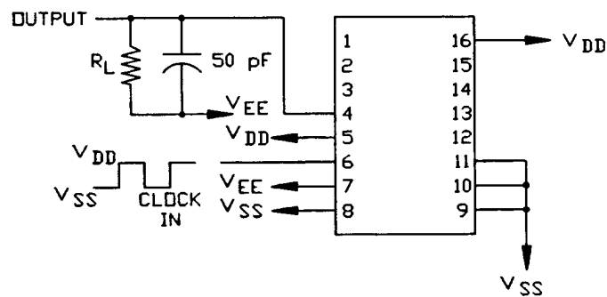
PROPAGATION DELAY, INHIBIT INPUT TO SIGNAL OUTPUT
