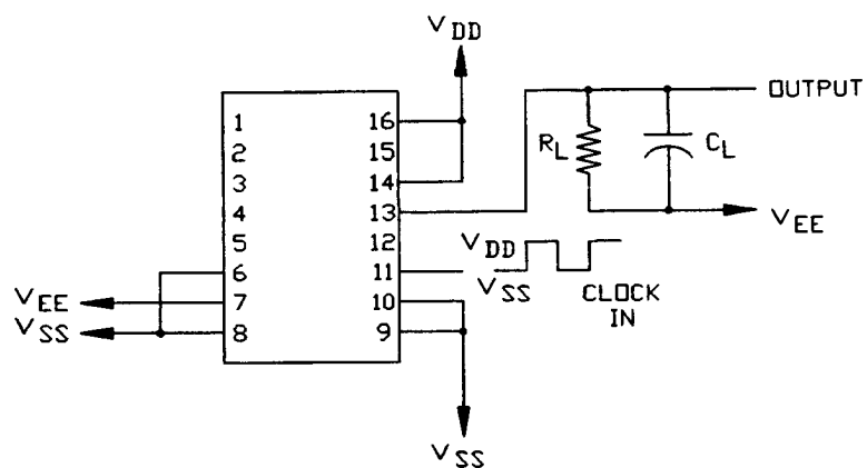
PROPAGATION DELAY, ADDRESS INPUT TO SIGNAL OUTPUT
