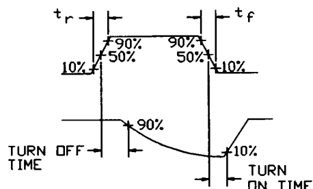
WAVEFORMS, CHANNEL BEING TURNED OFF.
