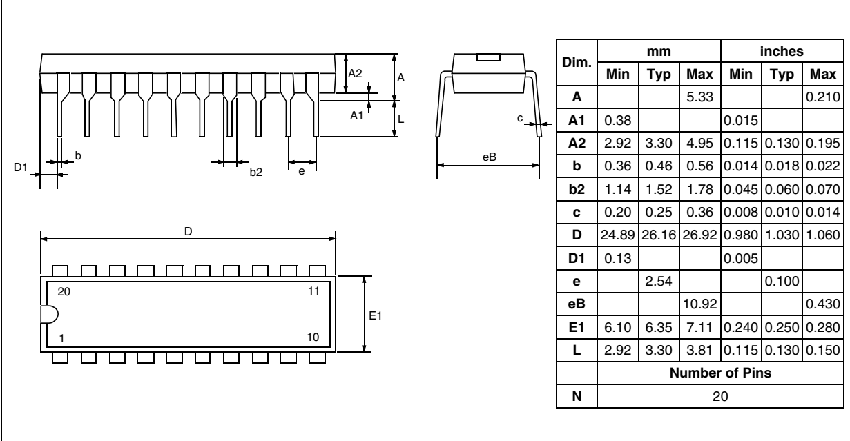
Figure 92. 20-Pin Plastic Dual In-Line Package, 300-mil Width
