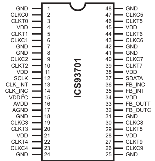
48-Pin TSSOP
