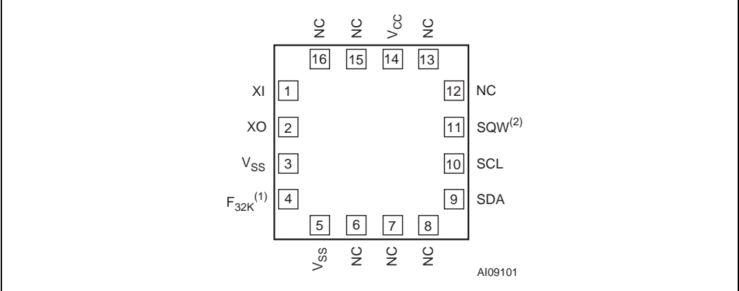
Figure 7. M41T64 connections
