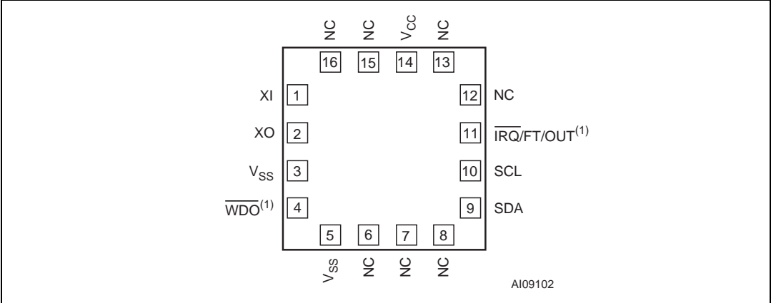
Figure 8. M41T65 connections
