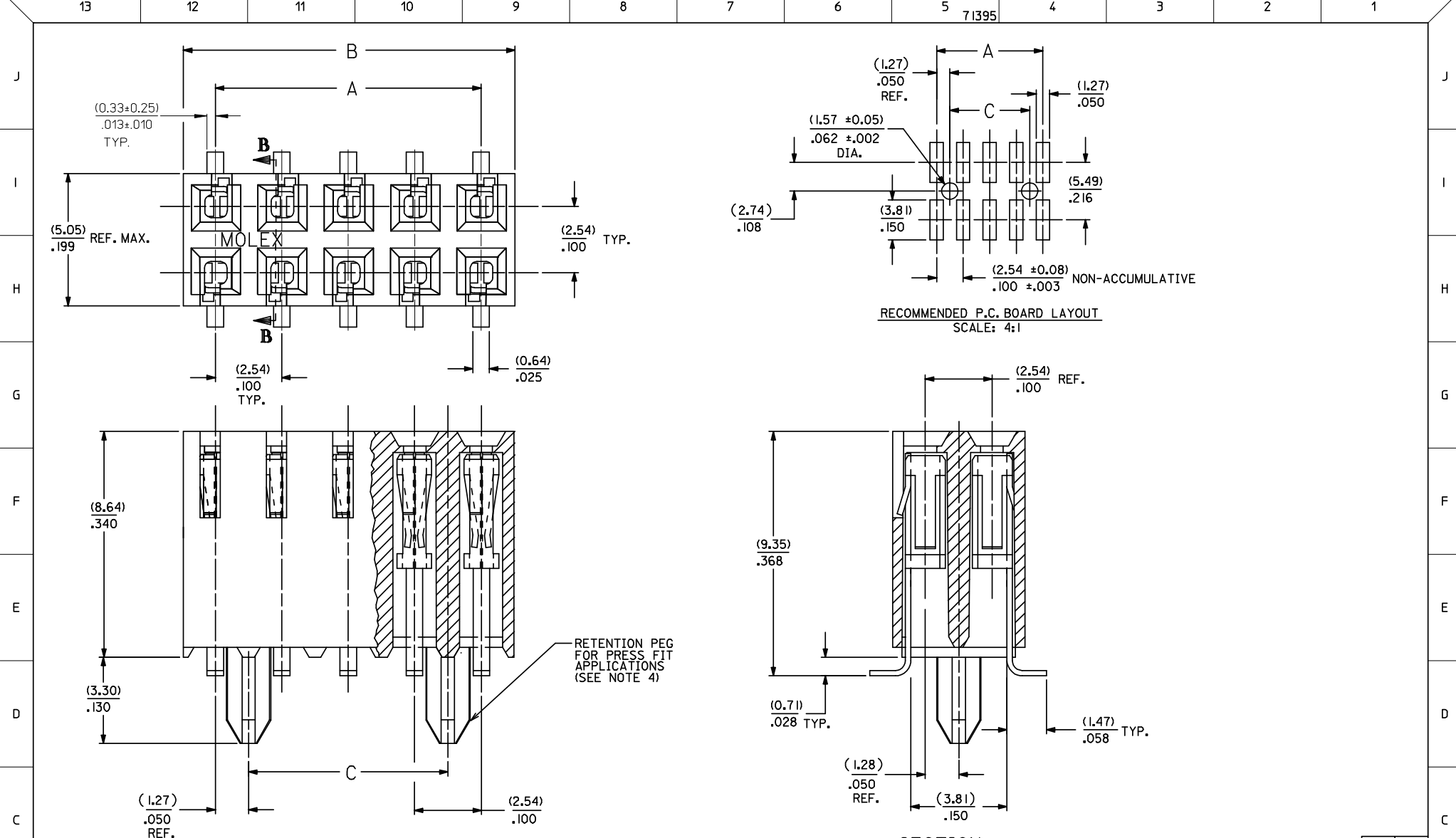
SECTION B-B - VERSION WITH PCB RETENTION PEGS -
