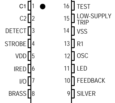
Figure 1. Pin Connections
