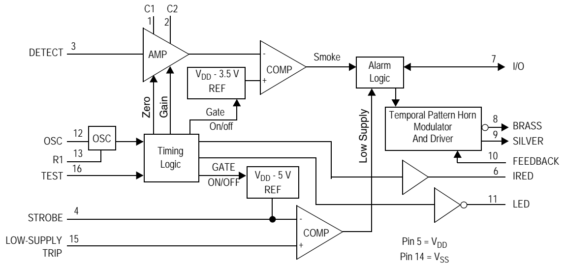
Figure 2. Block Diagram
