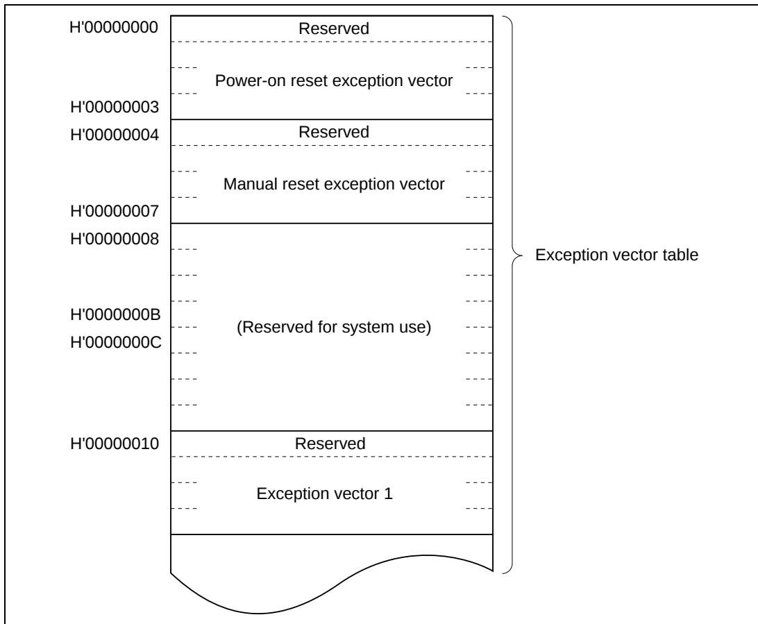
Figure 1.4 Exception Vector Table (Advanced Mode)
