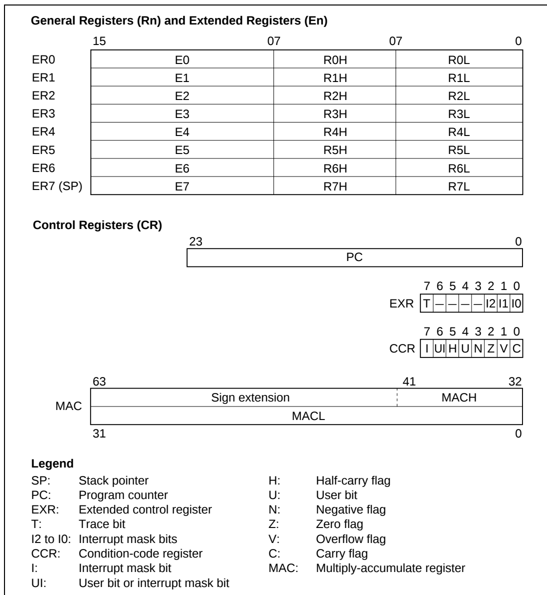
Figure 1.7 CPU Registers
