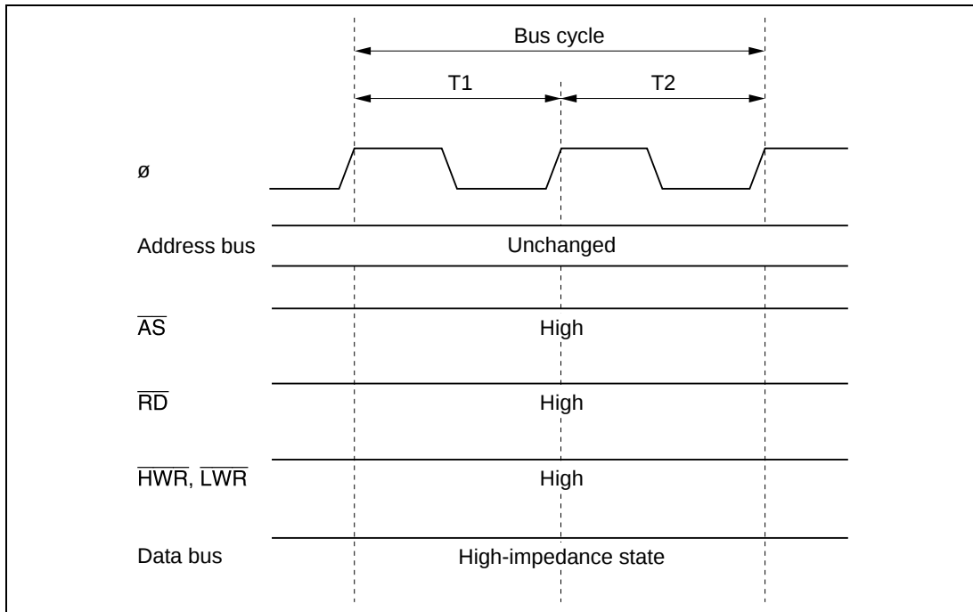
Figure 4.4 Pin States during On-Chip Supporting Module Access
