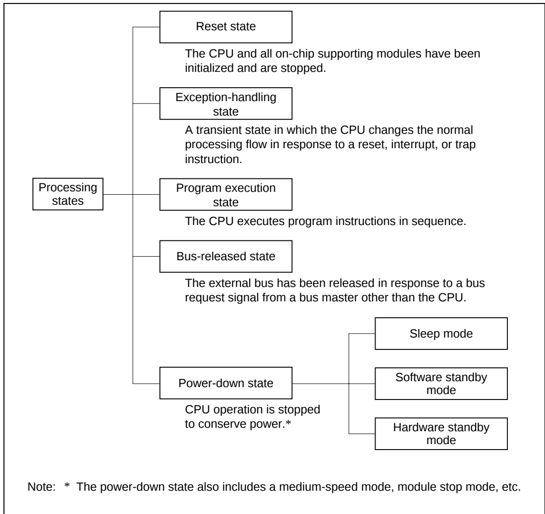
Figure 3.1 Processing States
