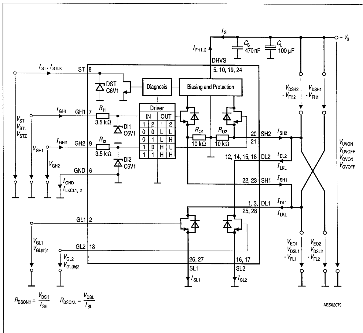
Figure 3 Test Circuit
