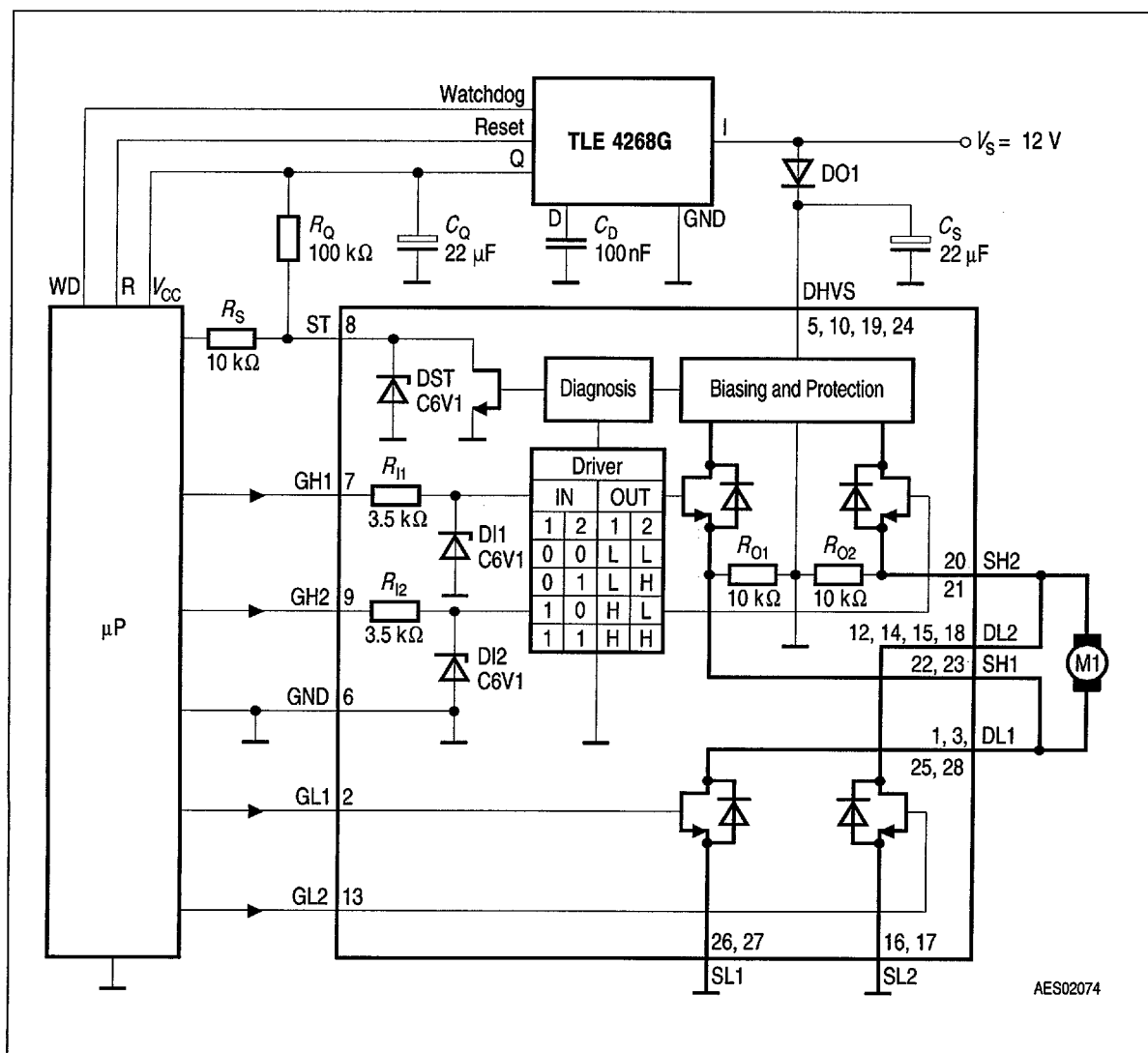
Figure 4 Application Circuit
