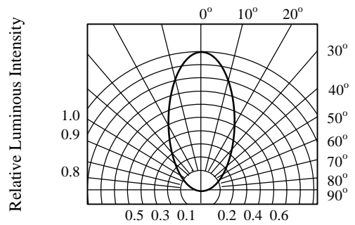
FIG.6 RADIATION DIAGRAM
