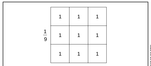
Figure 2 : Local Averaging Filter Kernel
