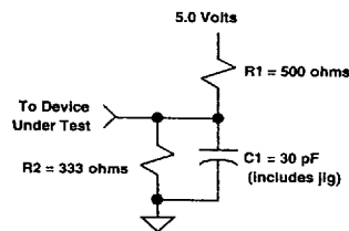
Fig. 2: TTL Switching Test Load
