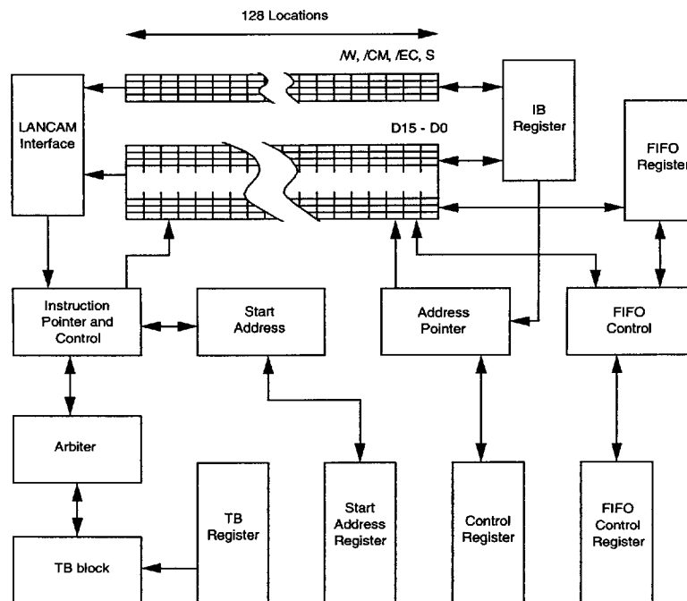
Figure 1: The Instruction Buffer
