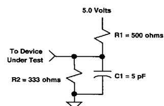
Fig. 3: Three-state Test Load
