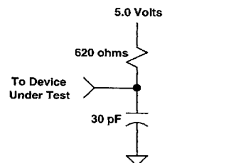
Fig. 4: Open-drain Test Load
