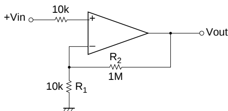
Figure 1 Noninverting Amplifier
