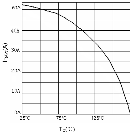
I_{F(AV)} vs T_C
