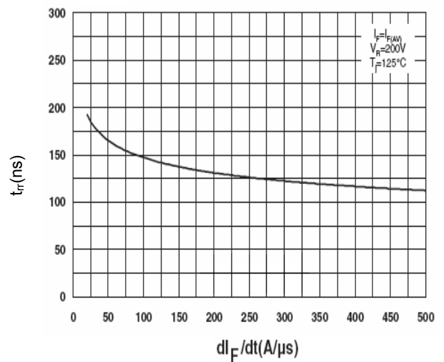
t_{rr} vs di_F/dt
