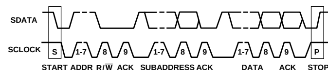
Figure 29. Bus Data Transfer
