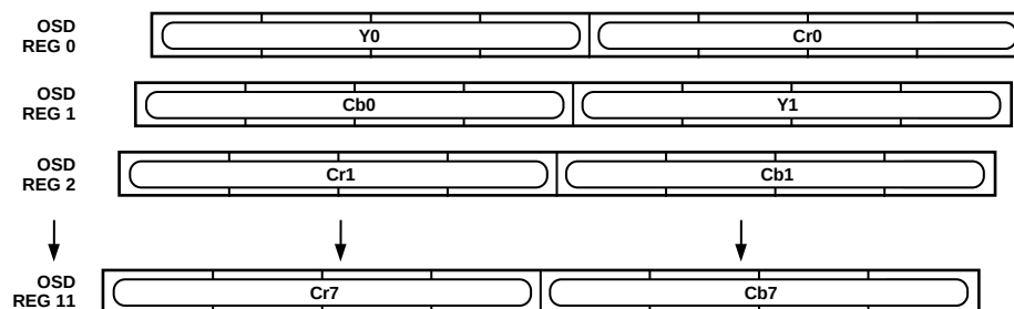
Figure 42. OSD Registers
