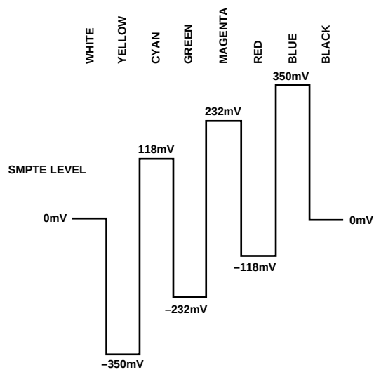
Figure 59. PAL 1005 Color Bars U Levels
