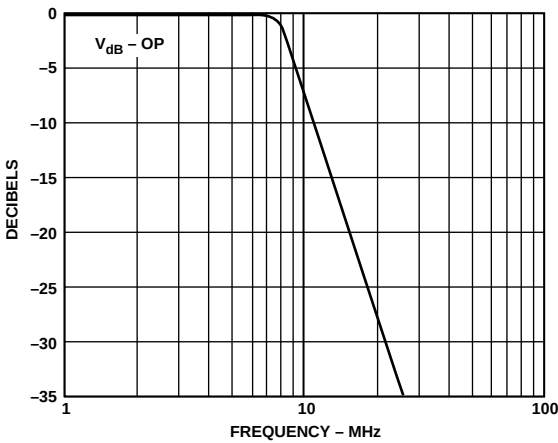
Figure 65. Output Filter Close Up
