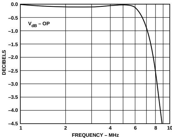
Figure 66. Output Filter Plot Close Up
