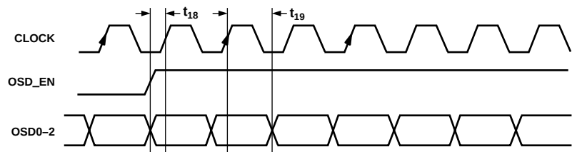
Figure 4. OSD Timing Diagram
