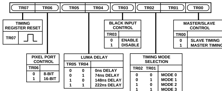
Figure 35. Timing Register 0
