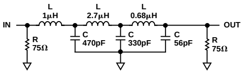
Figure 63. Output Filter
