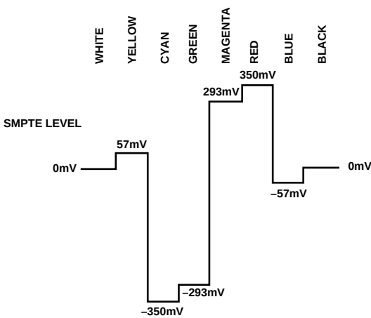
Figure 62. PAL 100% Color Bars V Levels
