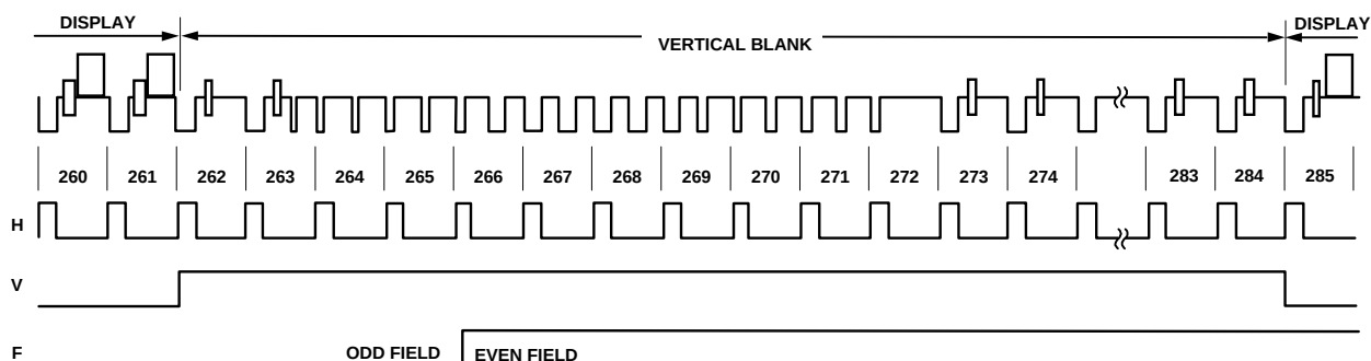
Figure 15. Timing Mode 0 (NTSC Master Mode)
