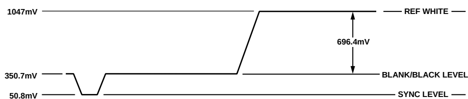
Figure 54. PAL Luma Video Levels
