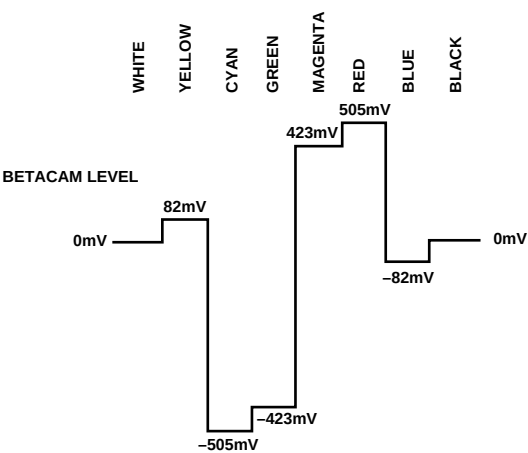
Figure 60. NTSC 100% Color Bars No Pedestal V Levels
