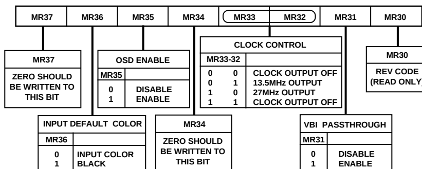
Figure 41. Mode Register 3
