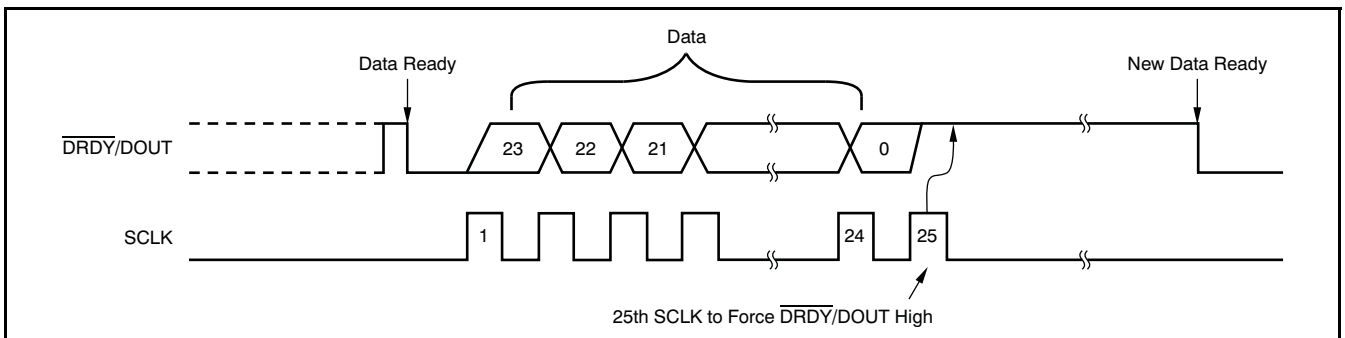
Figure 29. Data Retrieval with \overline{\text{DRDY}}/\text{DOUT} Forced High Afterwards
