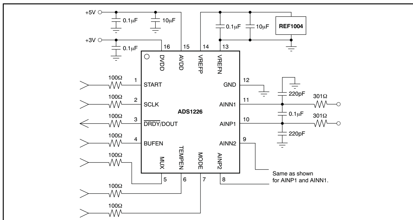
Figure 31. Basic Connections
