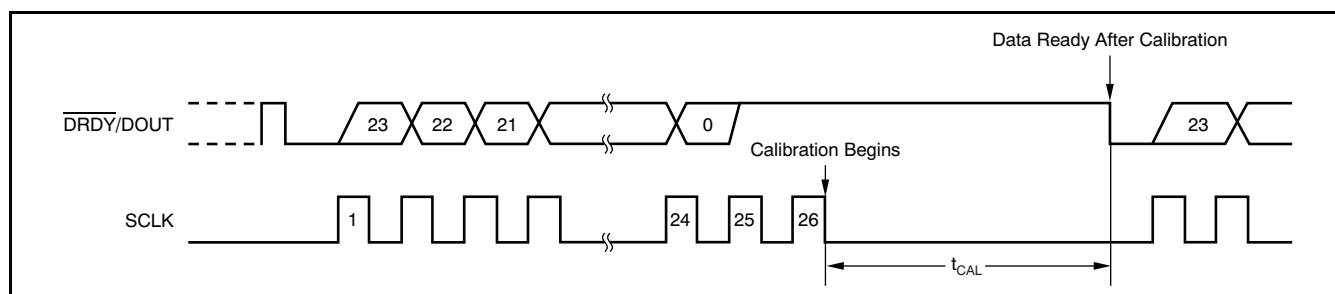
Figure 30. Self-Calibration Timing
