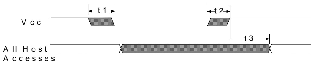
Figure 29.1 Power-Up Timing
