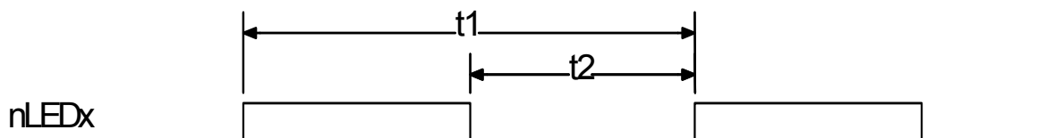
Figure 29.28 nLEDx Timing
