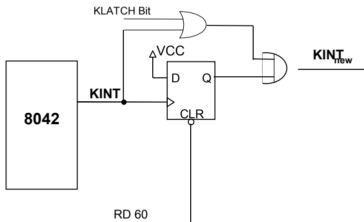
Figure 12.3 Keyboard Latch
