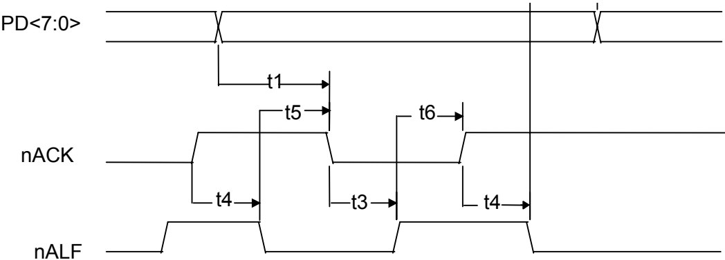
Figure 29.19 ECP Parallel Port Reverse Timing
