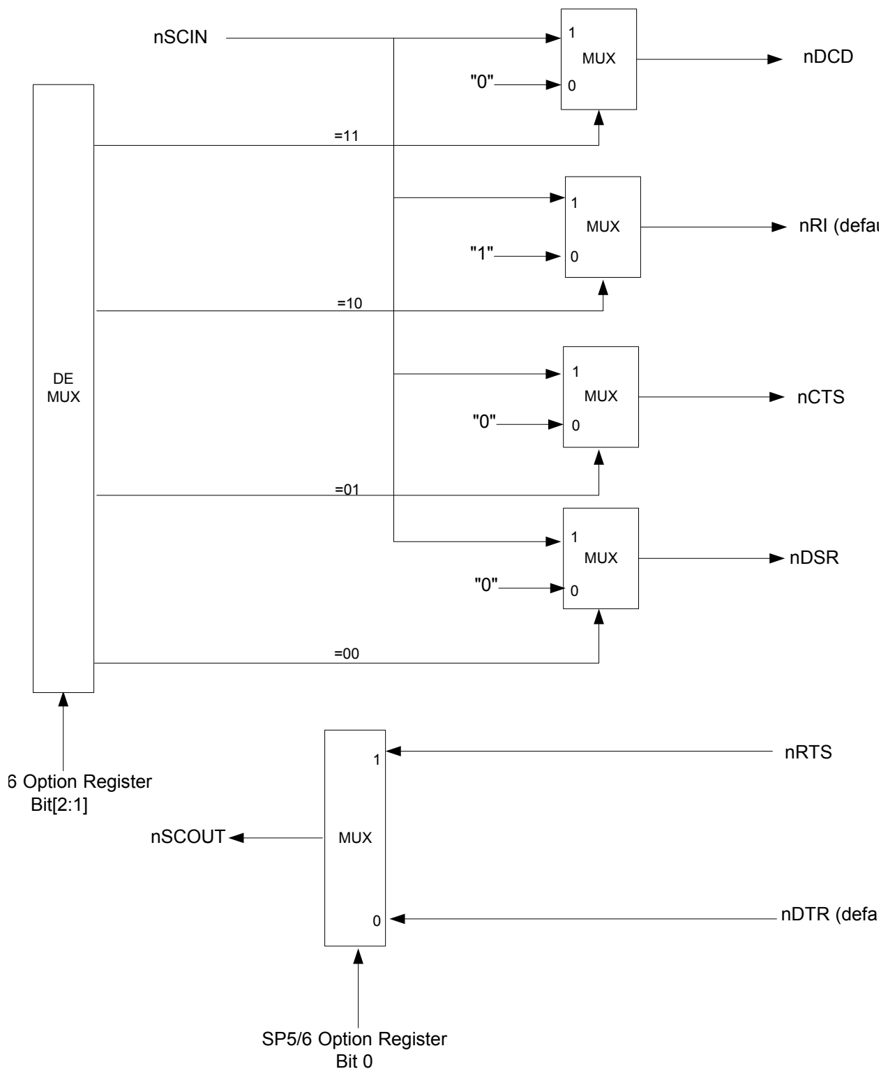
Figure 8.5 Reduce Pin Serial Port Control Signal Selection
