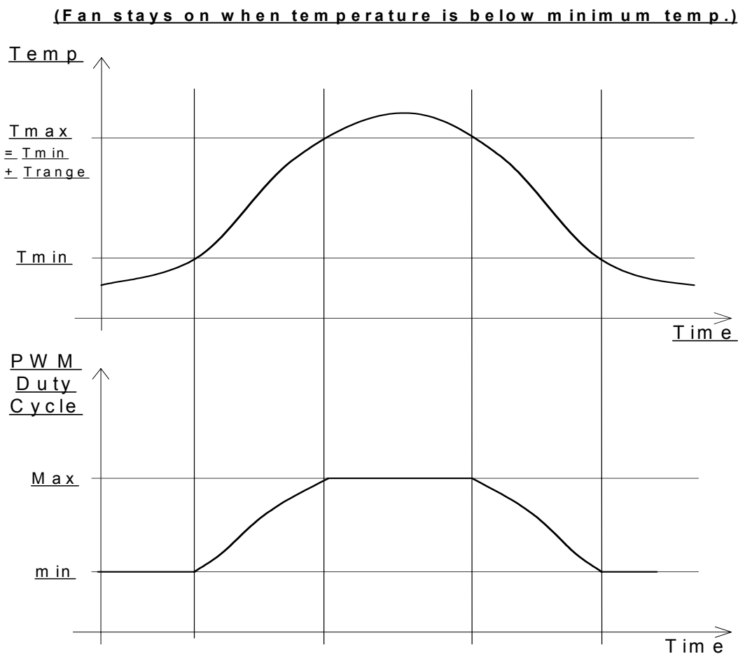
Figure 23.5 Automatic Fan Control
