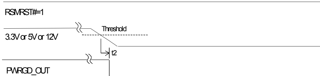
(b) Power Down Due to Drop in Power Supply
