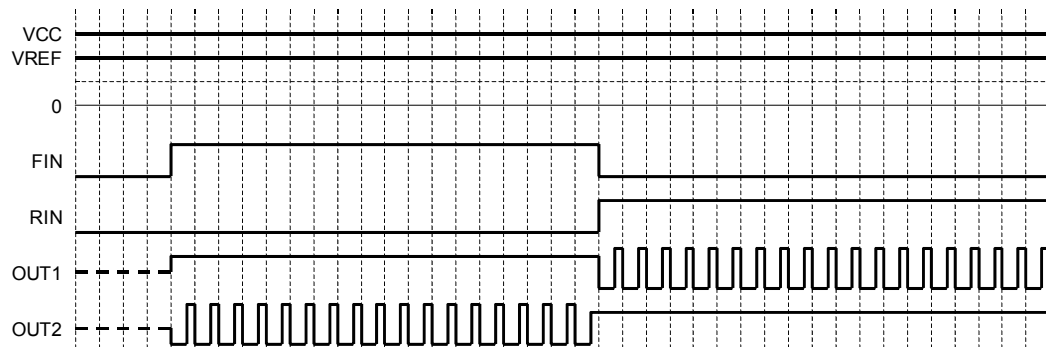
Fig.40 VREF control operation (timing chart)
