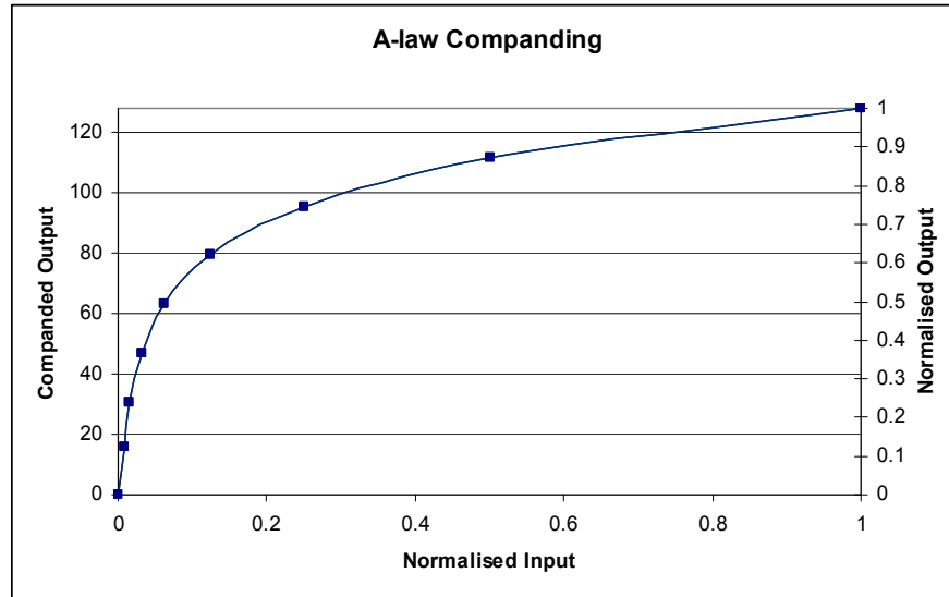
Figure 30 A-Law Companding
