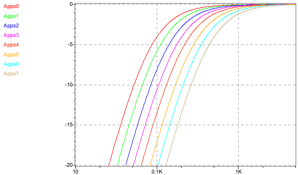
Figure 50 ADC High Pass Filter Frequency Response for the Application Mode (Sample rate, f_s = 48\text{kHz} )
