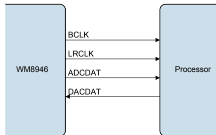
Figure 21 Master Mode
