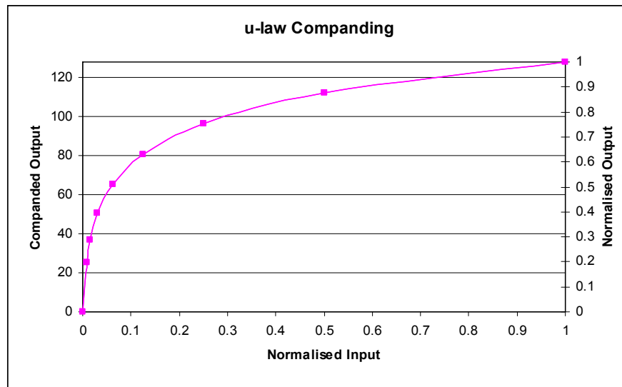
Figure 29 \mu -Law Companding
