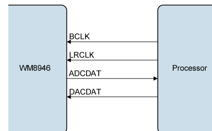
Figure 22 Slave Mode
