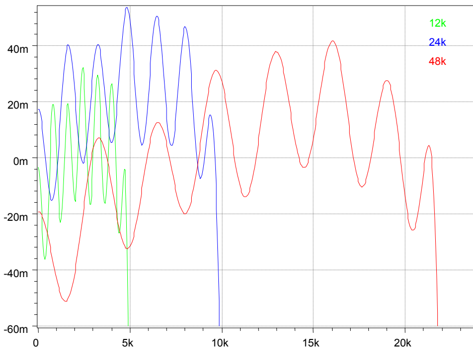
Figure 54 DAC Pass Band Frequency Response up to fs/2 (Sample rate, fs = 8k to 12kHz, 16k to 24kHz, 32k to 48kHz)
