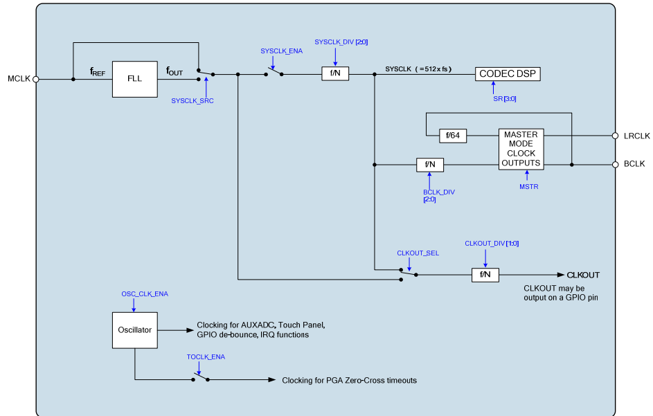
Figure 32 WM8946 Clocking Overview
