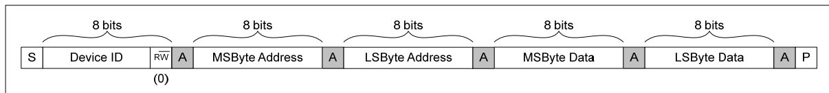
Figure 37 Single Register Write to Specified Address
