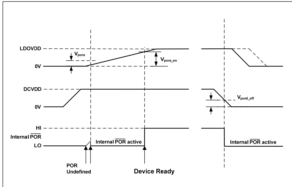
Figure 46 Power On Reset Timing – DCVDD Enabled First
