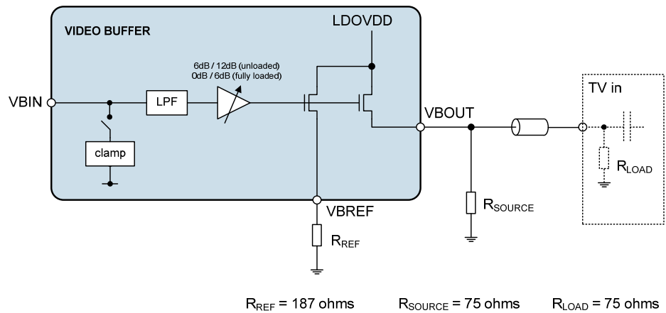
Figure 60 Typical Components for Video Buffer
