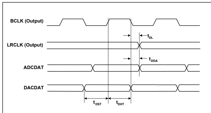
Figure 3 Audio Interface Timing - Master Mode
