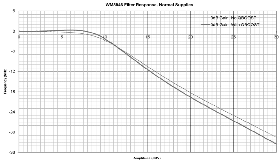
Figure 33 Video Buffer Lowpass Filter Frequency Response Gain=0dB
