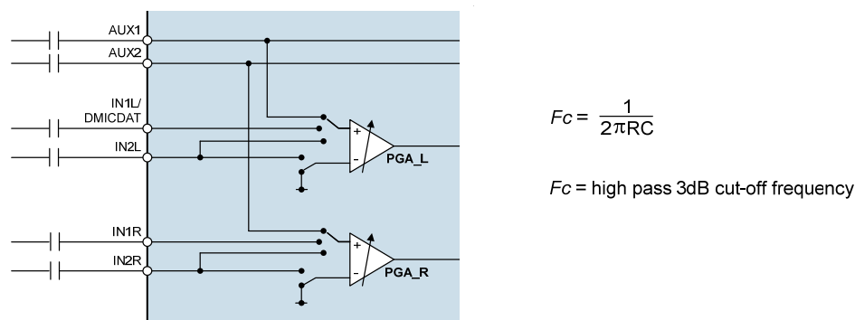
Figure 55 Audio Input Path DC Blocking Capacitor
