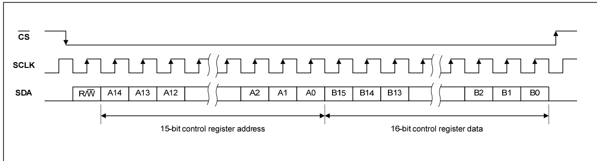
Figure 42 3-Wire Serial Control Interface
