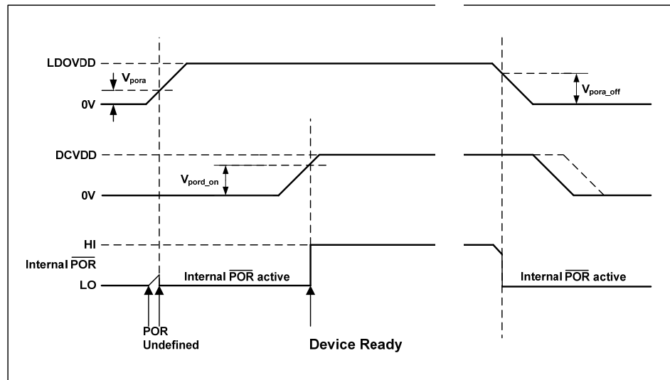
Figure 45 Power On Reset Timing – LDOVDD Enabled First
