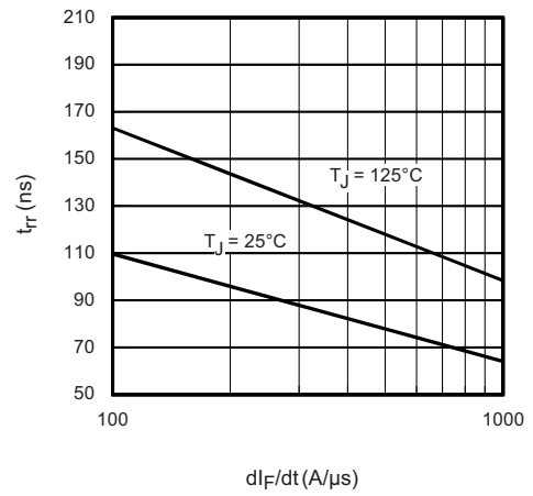
Fig. 13 - Typical t_{rr} diode vs. di/dt V_{RR} = 200\text{ V} , I_F = 50\text{ A}
