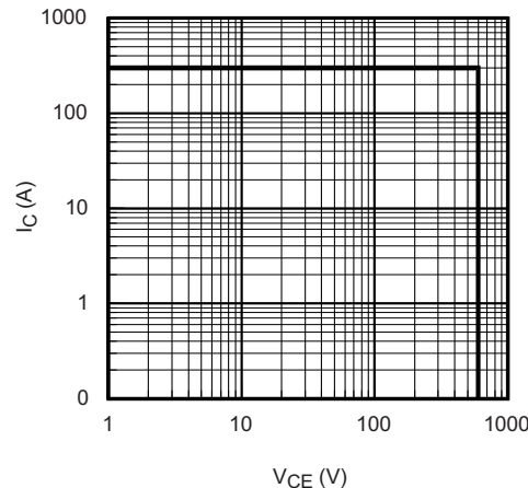
Fig. 2 - IGBT Reverse Bias SOA T_J = 150\text{ }^\circ\text{C}, V_{GE} = 15\text{ V}
