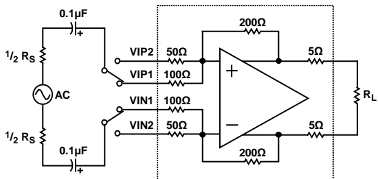
Figure 33. Differential Input Loading Circuit
