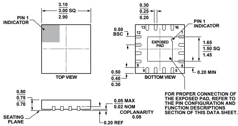
Figure 47. 16-Lead Lead Frame Chip Scale Package [LFCSP_WQ] 3 mm × 3 mm Body, Very Very Thin Quad (CP-16-27)
