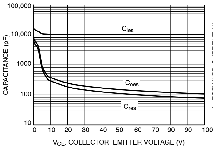
Figure 5. Typical Capacitance
