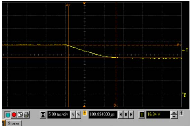
FIGURE 10. VLNb TRANSITIONS FROM 18.3V TO 13.3V
