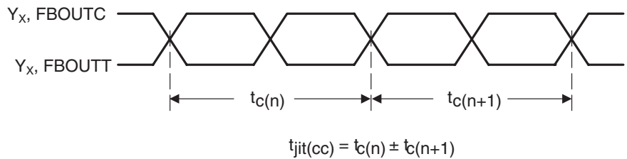
Figure 3. Cycle-to-Cycle Jitter
