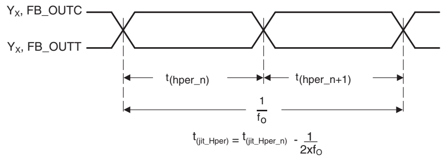
Figure 7. Half-Period Jitter
