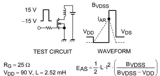
Fig. 8.16 Test Circuit/Waveform
