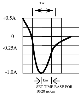
FIG. 1-TEST CIRCUIT DIAGRAM AND REVERSE RECOVERY TIME CHARACTERISTIC
