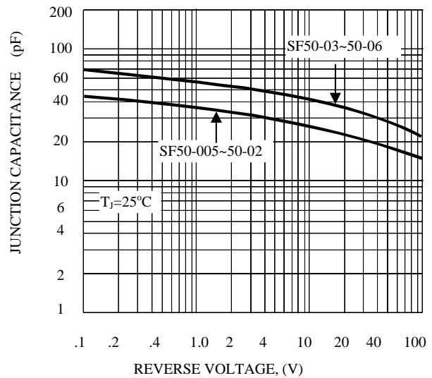
FIG. 6-TYPICAL JUNCTION CAPACITANCE
