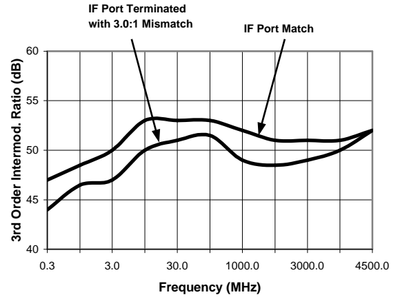
3rd Order IM Ratio - Input +7 dBm
