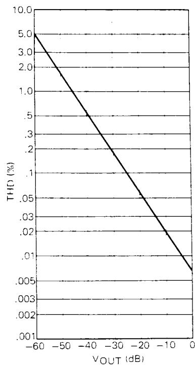
Fig. 4 Total Harmonic Distortion (THD) VS V_{OUT}
