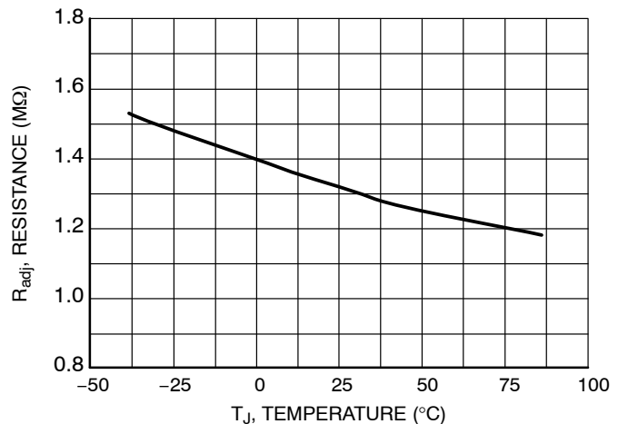
Figure 4. ADJ Pin Resistance vs. Temperature
