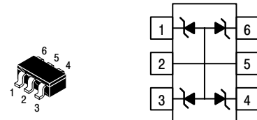
SC-59 PLASTIC CASE 318F
