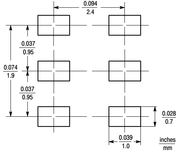
SC-59 6 LEAD
