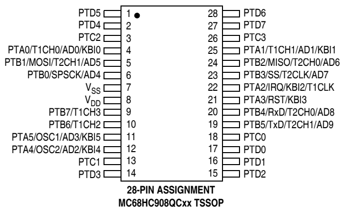
Figure 1-2. MC68HC908QC16, MC68HC908QC8, and MC68HC908QC4 Pin Assignments
