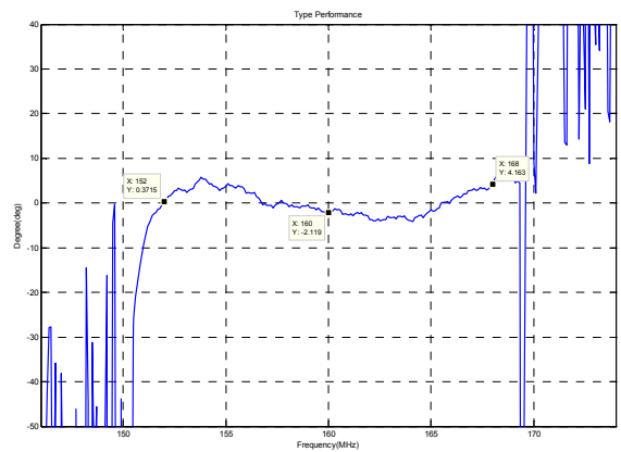
Phase Linearity( f_0 \pm 8\text{MHz} )
