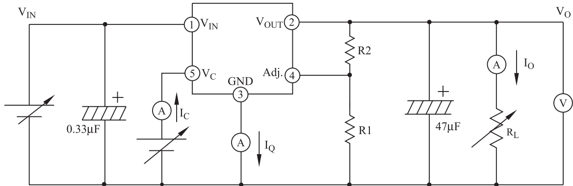
Fig. 1 Test Circuit
