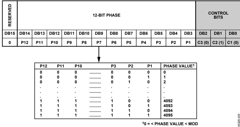
Figure 31. Phase Register (R2)
