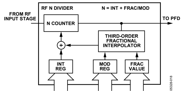
Figure 22. Fractional-N Divider
