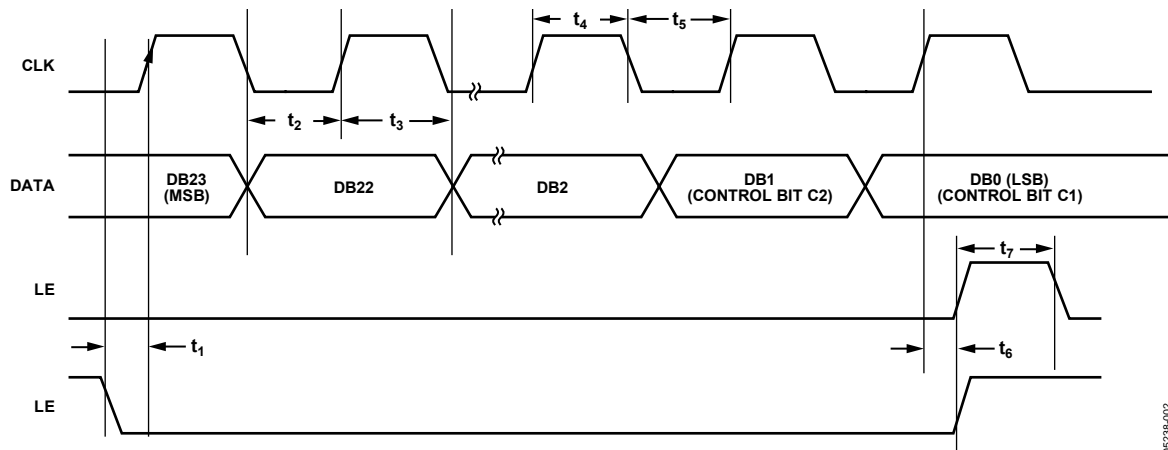
Figure 2. Timing Diagram
