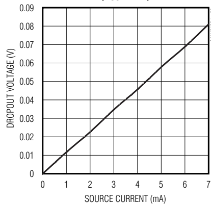
DROPOUT VOLTAGE vs. SOURCE CURRENT ( V_{OUT} = 5V )
