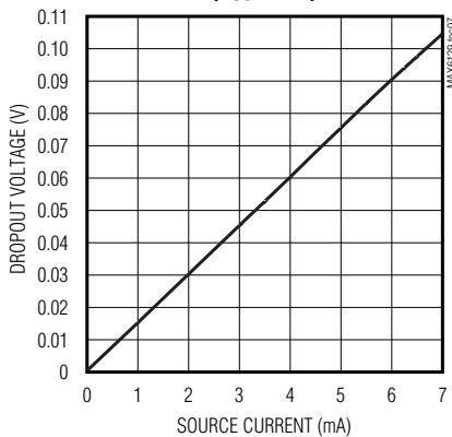
DROPOUT VOLTAGE vs. SOURCE CURRENT ( V_{OUT} = 3V )
