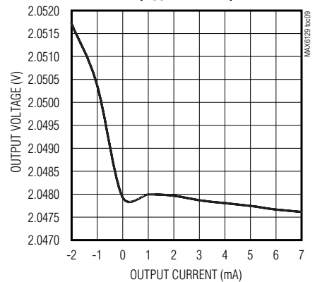
LOAD REGULATION ( V_{OUT} = 2.048V )
