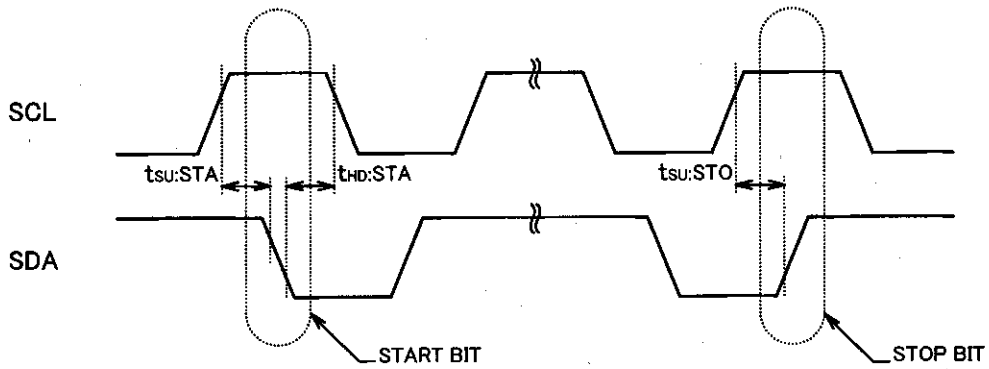
Fig.-4 SYNCHRONOUS DATA TIMING
