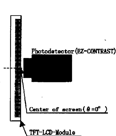
Fig2-1 Viewing angle measurement method
