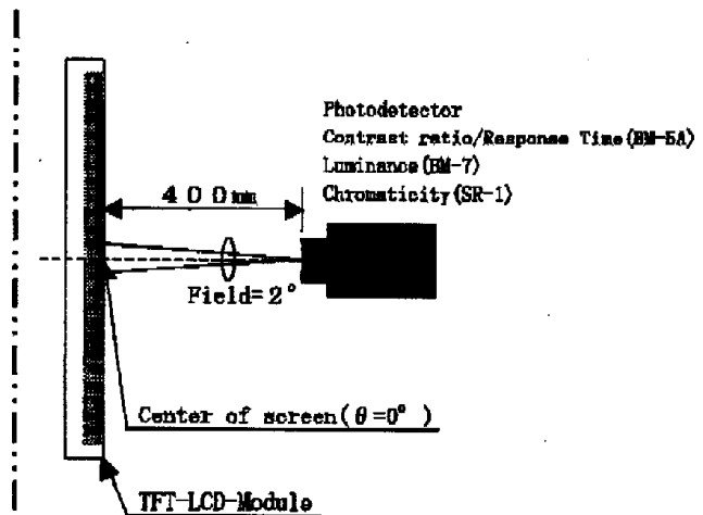
Fig2 -2 Luminance/Contrast ratio/Response time/Chromaticity
