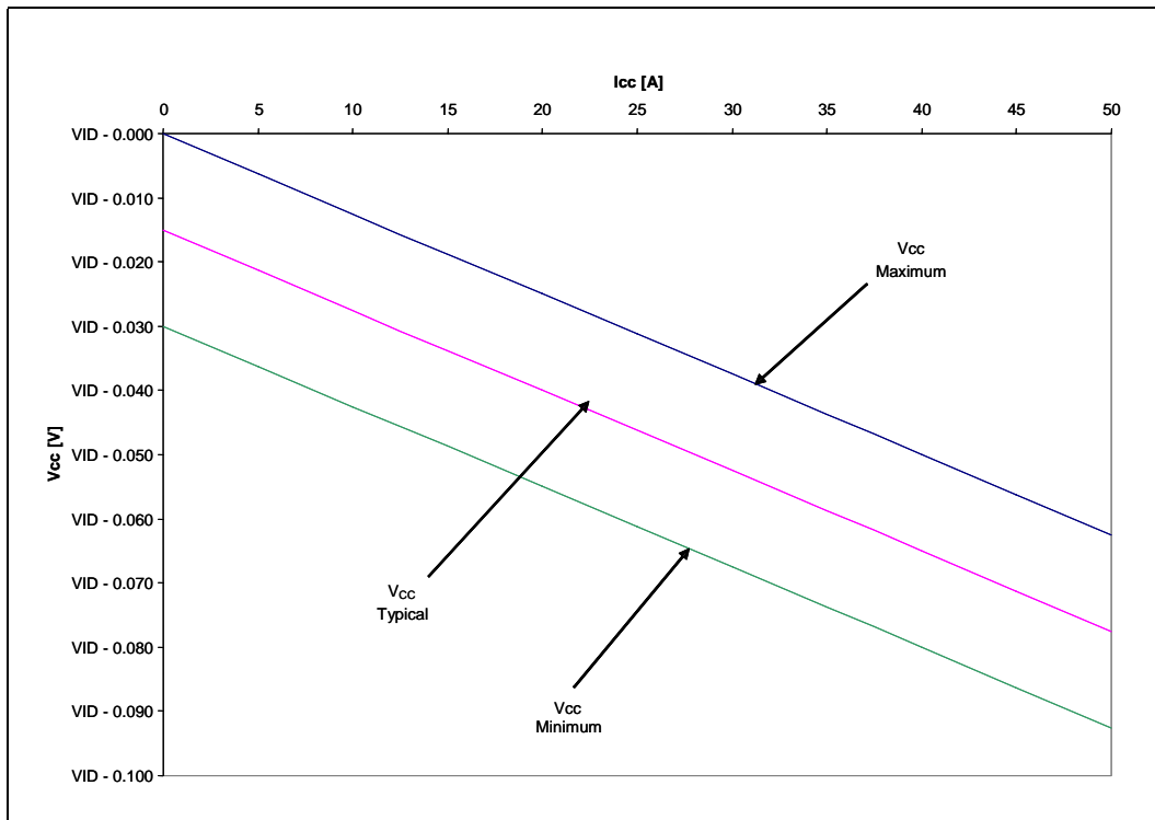
Figure 2-6. V CC Static and Transient Tolerance Load Lines
