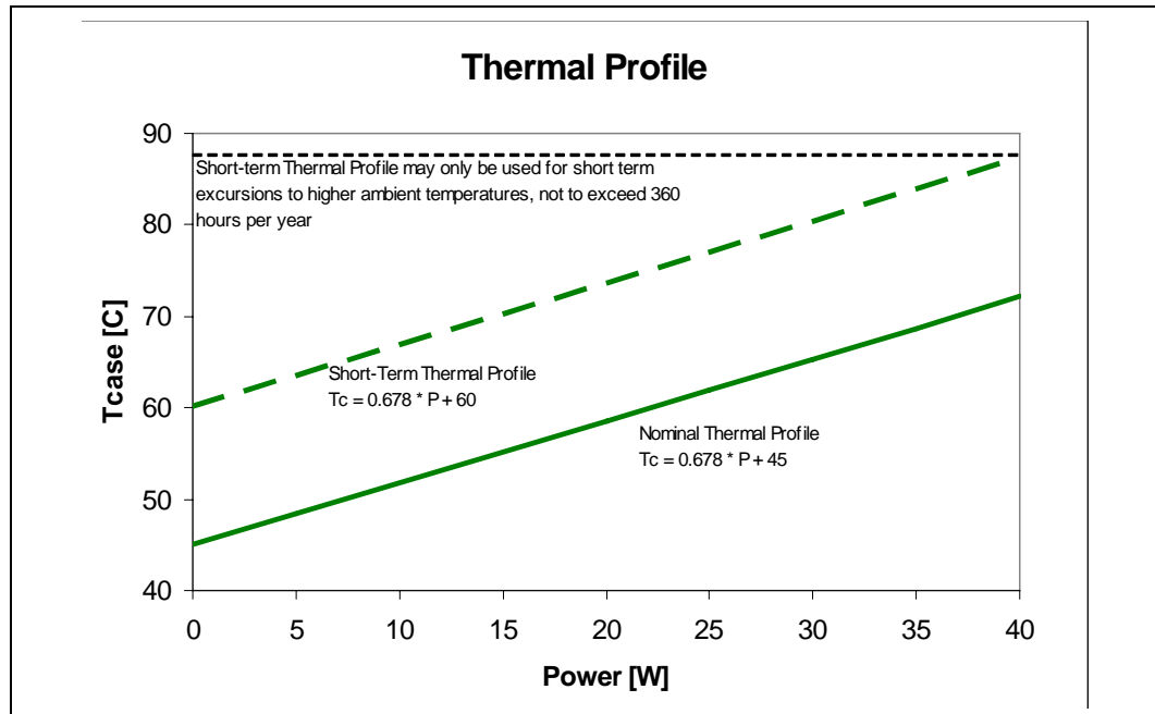
Figure 6-5. Quad-Core Intel® Xeon® Processor L5408 Thermal Profile
