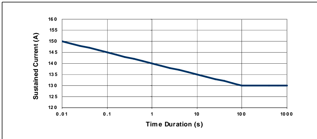
Figure 2-2. Quad-Core Intel® Xeon® Processor X5482 Load Current versus Time
