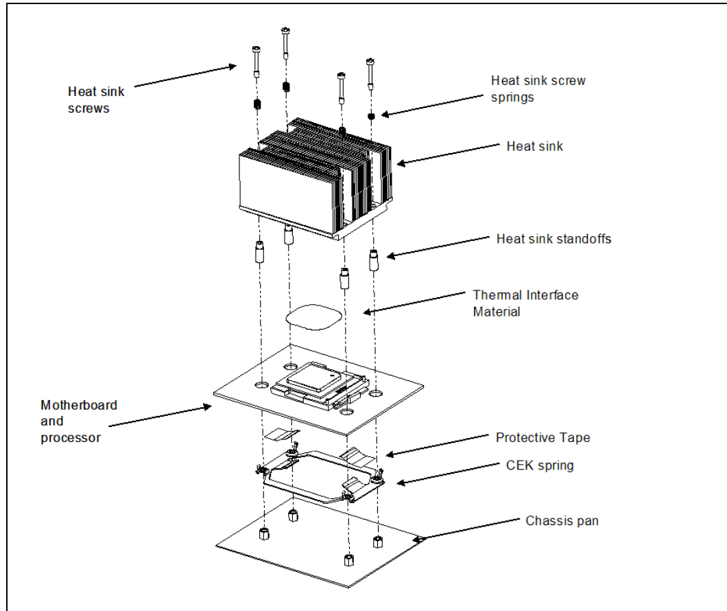
Figure 8-3. 2U Passive Quad-Core Intel® Xeon® Processor 5400 Series Thermal Solution (Exploded View)
