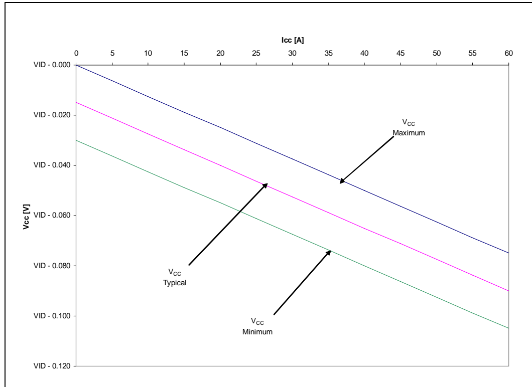
Figure 2-10. Quad-Core Intel® Xeon® Processor L5400 Series VCC Static and Transient Tolerance Load Lines
