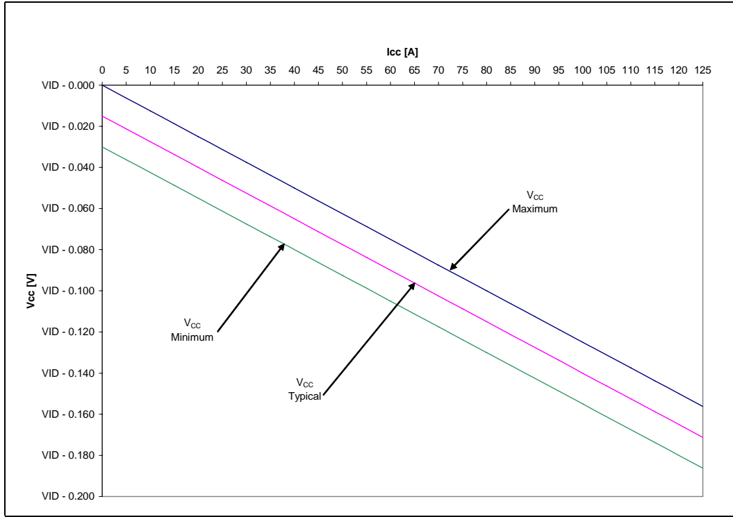
Figure 2-9. Quad-Core Intel® Xeon® Processor E5400 Series V_{CC} Static and Transient Tolerance Load Lines
