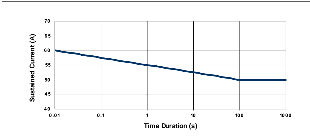
Figure 2-5. Quad-Core Intel® Xeon® Processor L5400 Series Load Current versus Time
