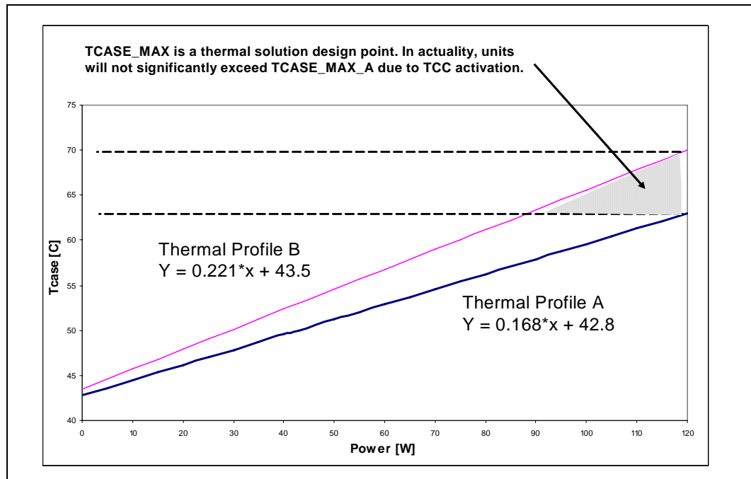
Figure 6-2. Quad-Core Intel® Xeon® Processor X5400 Series Thermal Profiles A and B
