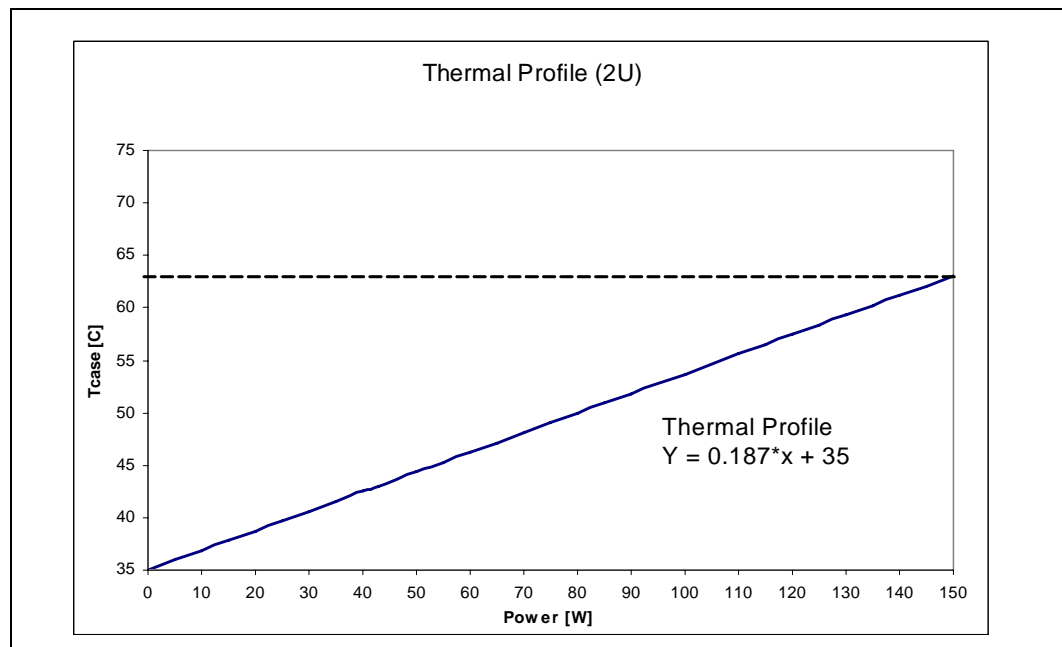
Figure 6-1. Quad-Core Intel® Xeon® Processor X5492 and X5482 (C-step) Thermal Profile
