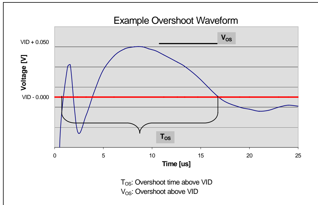
Figure 2-11. V_{CC} Overshoot Example Waveform
