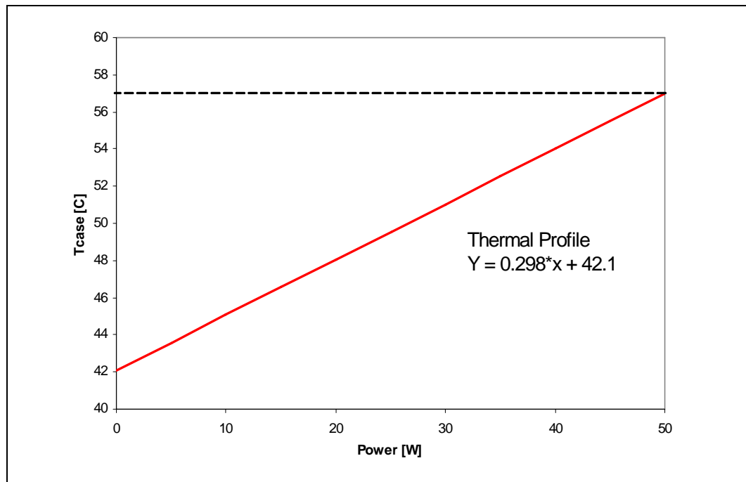
Figure 6-4. Quad-Core Intel® Xeon® Processor L5400 Series Thermal Profile
