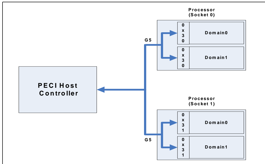
Figure 6-8. Quad-Core Intel® Xeon® Processor 5400 Series PECI Topology
