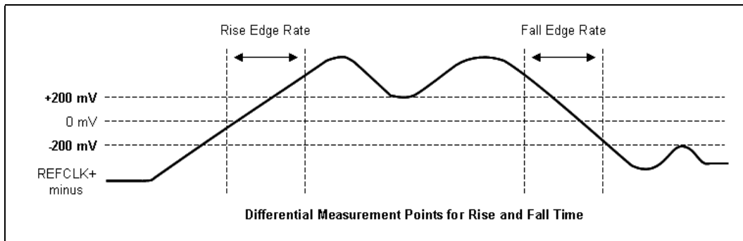
Figure 2-15. Differential Rising and Falling Edge Rates
