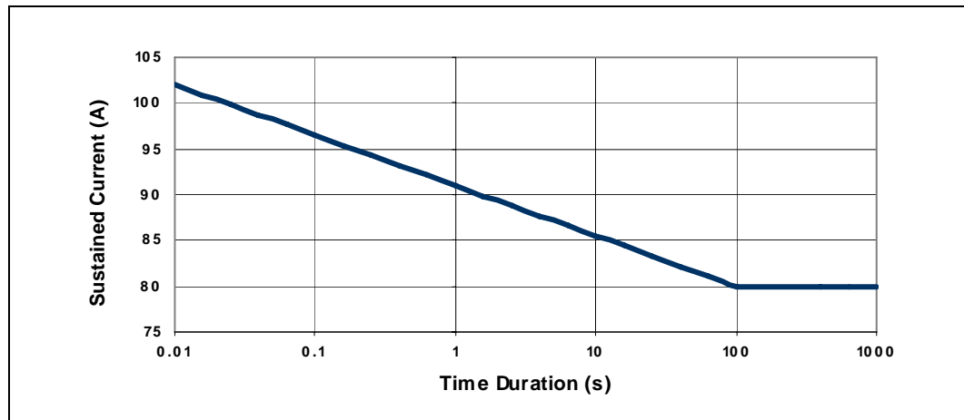
Figure 2-4. Quad-Core Intel® Xeon® Processor E5400 Series Load Current versus Time
