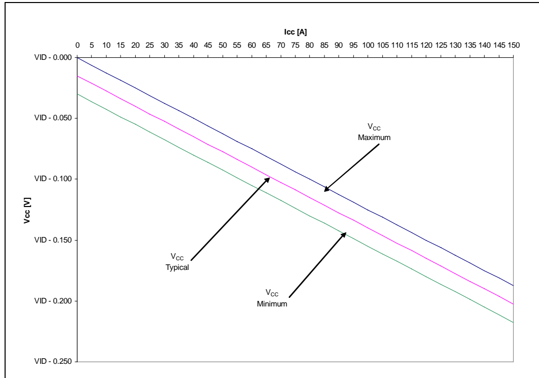
Figure 2-7. Quad-Core Intel® Xeon® Processor X5482 V_{CC} Static and Transient Tolerance Load Lines
