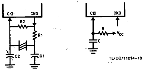
FIGURE 6. Crystal and R/C Oscillator Diagrams
