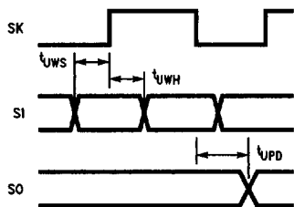
FIGURE 2. MICROWIRE/PLUS Timing
