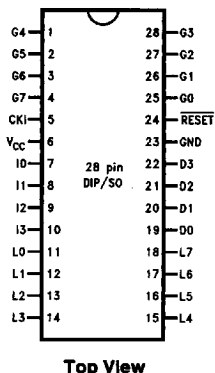
Dual-In-Line Package
