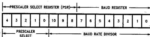
FIGURE 14. UART BAUD Clock Divisor Registers
