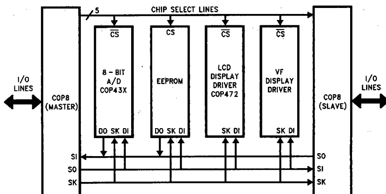
FIGURE 17. MICROWIRE/PLUS Application
