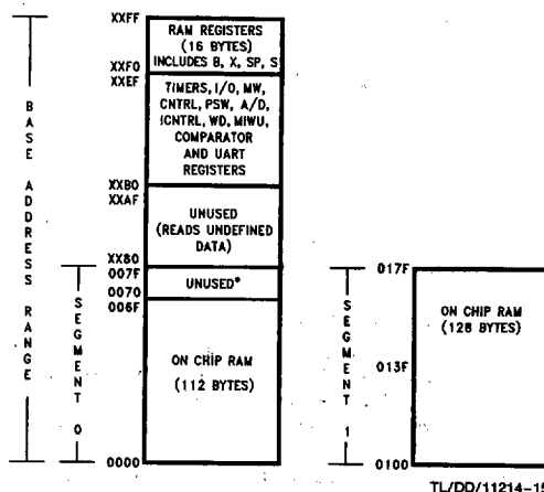
FIGURE 4. RAM Organization
