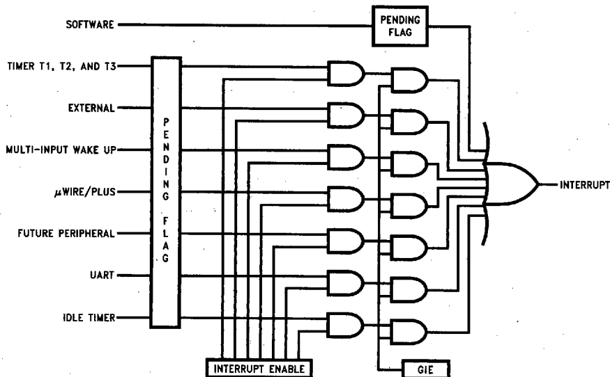
FIGURE 15. Interrupt Block Diagram
