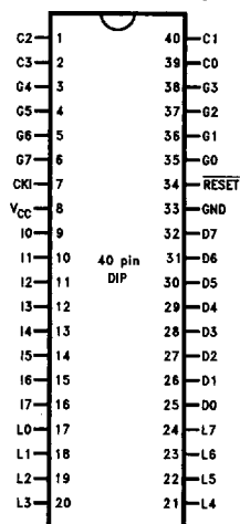
Dual-In-Line Package
