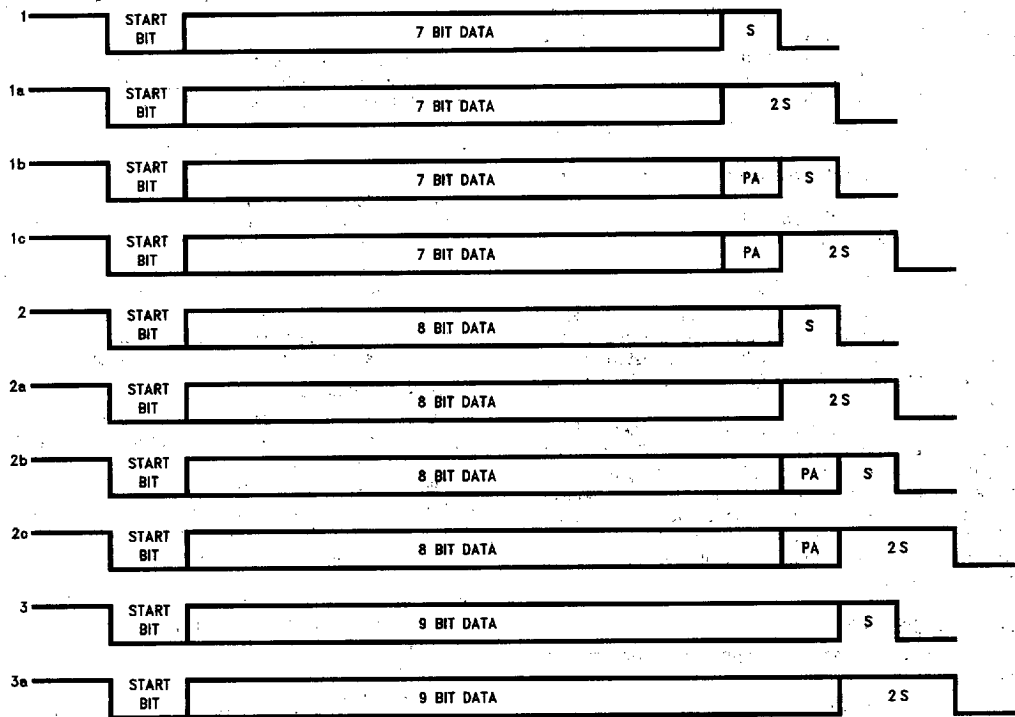
FIGURE 12. Framing Formats
