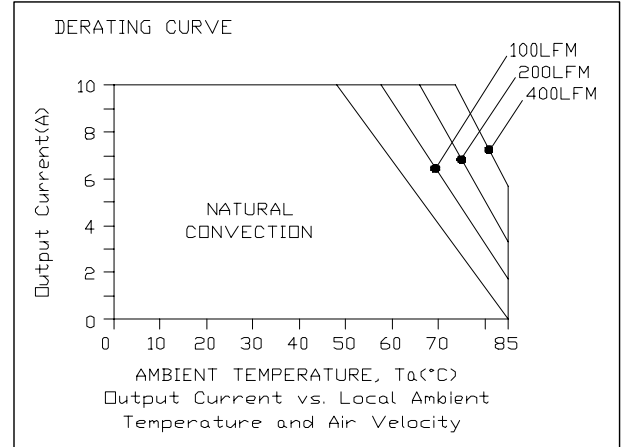
Derating curve under 48Vdc input
