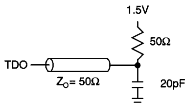
Figure 7 TAP AC OUTPUT LOAD EQUIVALENT
