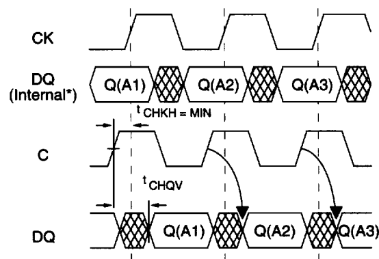
Figure 2 DUAL CLOCK MODE WITH t_{CHKH} = \text{MIN}
