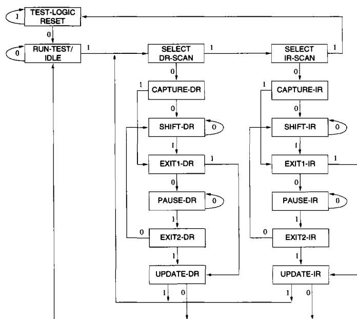
Figure 5 TAP CONTROLLER STATE DIAGRAM
