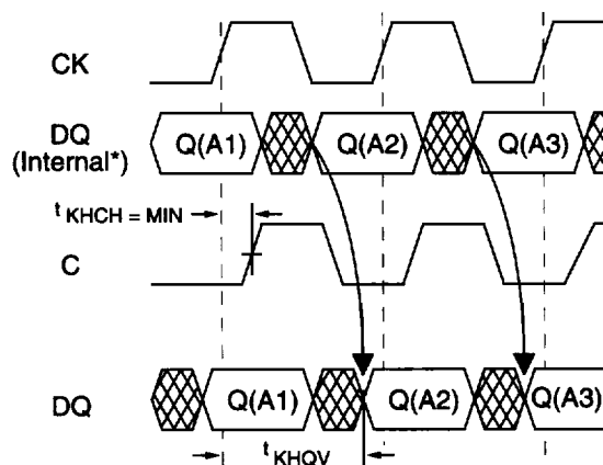
Figure 1 DUAL CLOCK MODE WITH t_{KHCH} = \text{MIN}
