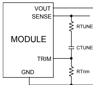
Figure 41. Circuit diagram showing connection of R_{TUNE} and C_{TUNE} to tune the control loop of the module.
