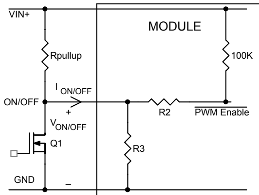
Figure 37. Circuit configuration for using negative On/Off logic.
