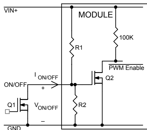
Figure 36. Circuit configuration for using positive On/Off logic.
