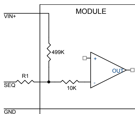
Figure 40. Circuit showing connection of the sequencing signal to the SEQ pin.
