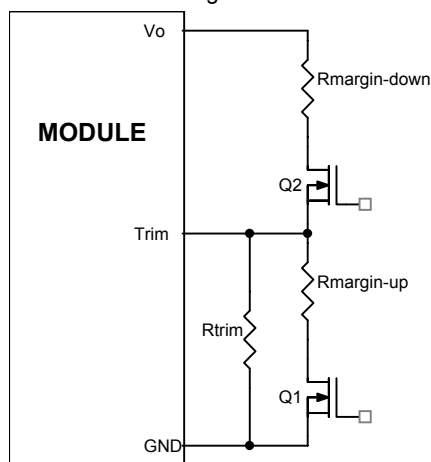
Figure 39. Circuit Configuration for margining Output voltage.
