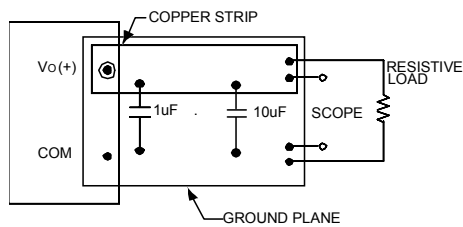
Figure 31. Input Reflected Ripple Current Test Setup.
