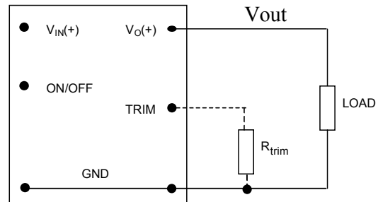
Figure 38. Circuit configuration for programming output voltage using an external resistor.
