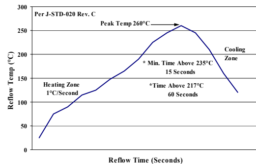
Figure 44. Recommended linear reflow profile using Sn/Ag/Cu solder.
