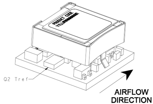
Figure 43. Preferred airflow direction and location of hot-spot of the module ( T_{ref} ).
