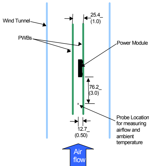
Figure 42. Thermal Test Setup.
