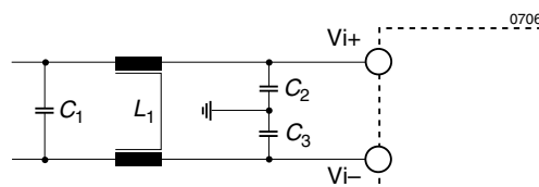
Fig. 4 Input filter arrangement for 48 V DC types
