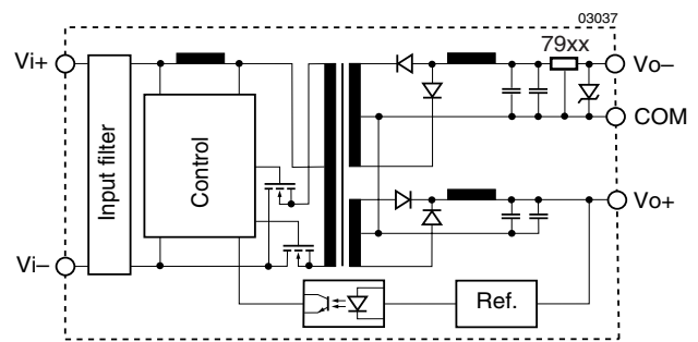
Fig. 2 Dual output converter block diagram
