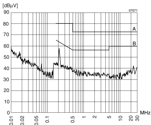
Fig. 6 Conducted RFI at input according to EN 55022 e.g. 48 IMR 40-24-2. U_i = 48 V DC.
