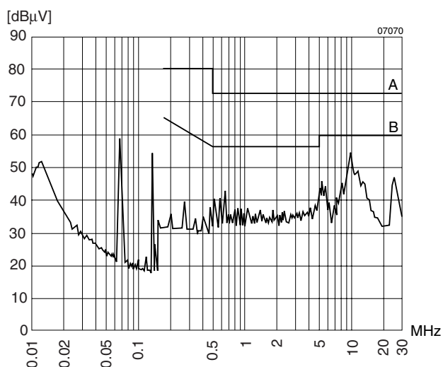
Fig. 5 Conducted RFI at input according to EN 55022 e.g. 12 IMR 40-24-2. U_i = 12 V DC.
