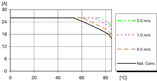
Available load current vs. ambient air temperature and airflow at V_I = 12.0\text{ V} , V_{OUT} = 1.8\text{ V} . See Thermal Consideration section.
