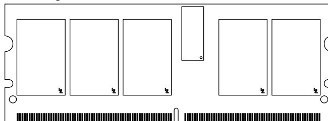
Figure 1: 244-Pin Mini-RDIMM (MO-244 R/C X)
