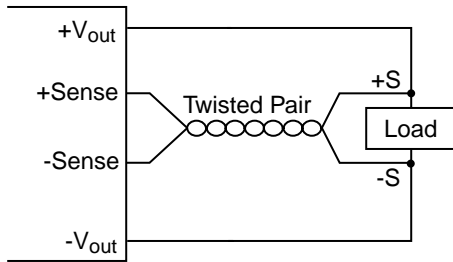
Fig.8 Sense Connections
